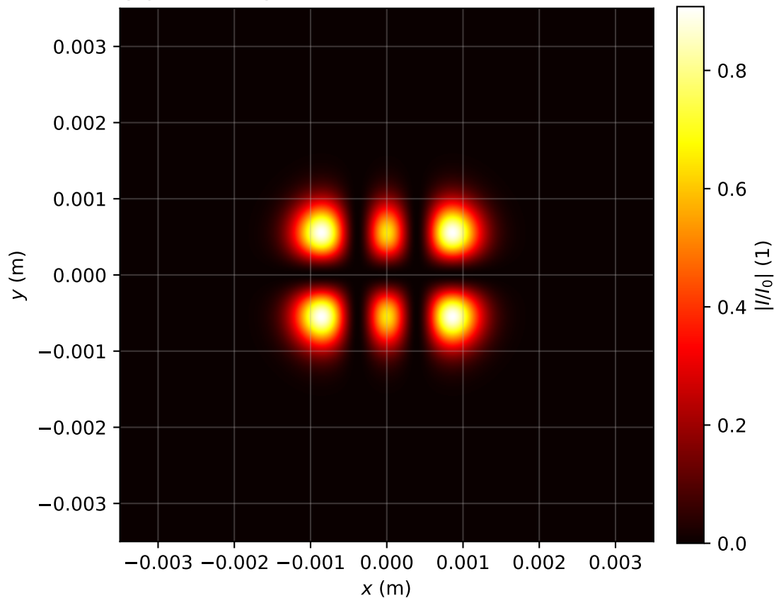
Intensity profile I(x, y, z = 0.876)/I_0 , P_{in}=0.5P_{cr} , artificial time
